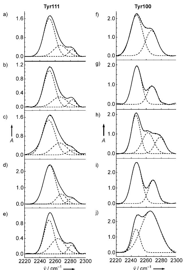
Figure 2. Spectra and fits of [D_4] Tyr111 (left) and [D_4] Tyr100 (right). a,f) Apo DHFR, b,g) NADPH complex, c,h) folate/ NADP^+ complex, d,i) MTX/NADPH complex, e,j) folate complex.
